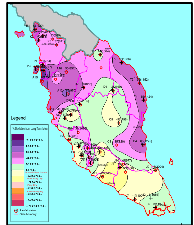
STATUS OF WATER RESOURCES In PENINSULAR MALAYSIA BASED On RAINFALL CUMULATIVE ANALYSIS YEAR 2009 PERIOD 6 month : 12_2008 & 1,2,3,4,5
