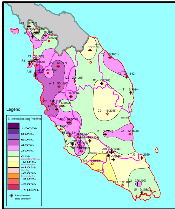
STATUS OF WATER RESOURCES In PENINSULAR MALAYSIA BASED On RAINFALL CUMULATIVE ANALYSIS YEAR 2009 PERIOD 6 month :10,11,12_2008 & 1,2,3_2009
