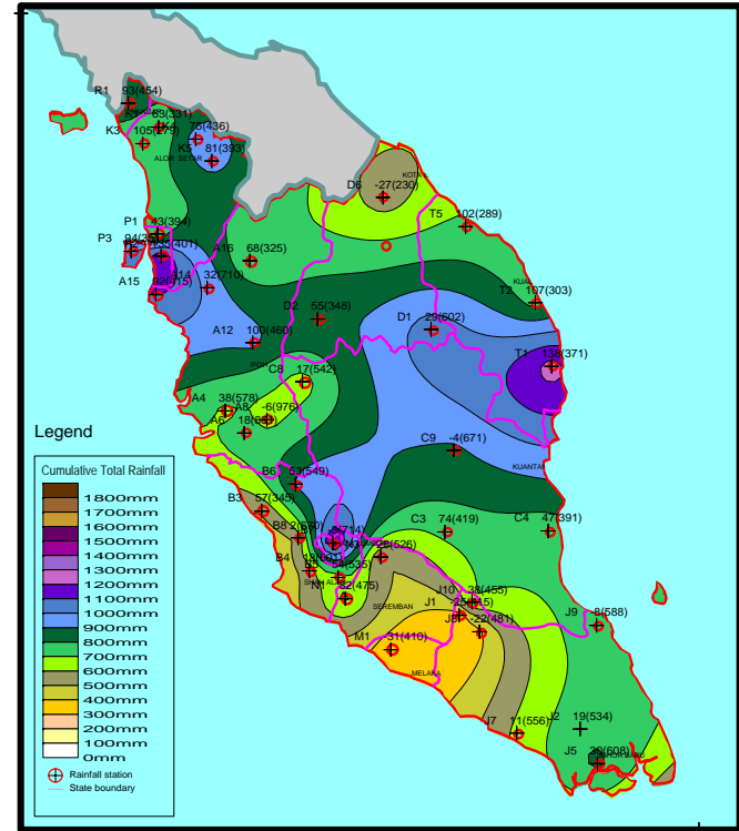
CUMULATIVE RAINFALL DISTRIBUTION IN PENINSULAR MALAYSIA YEAR 2009 PERIOD 3 month : 3,4,5
