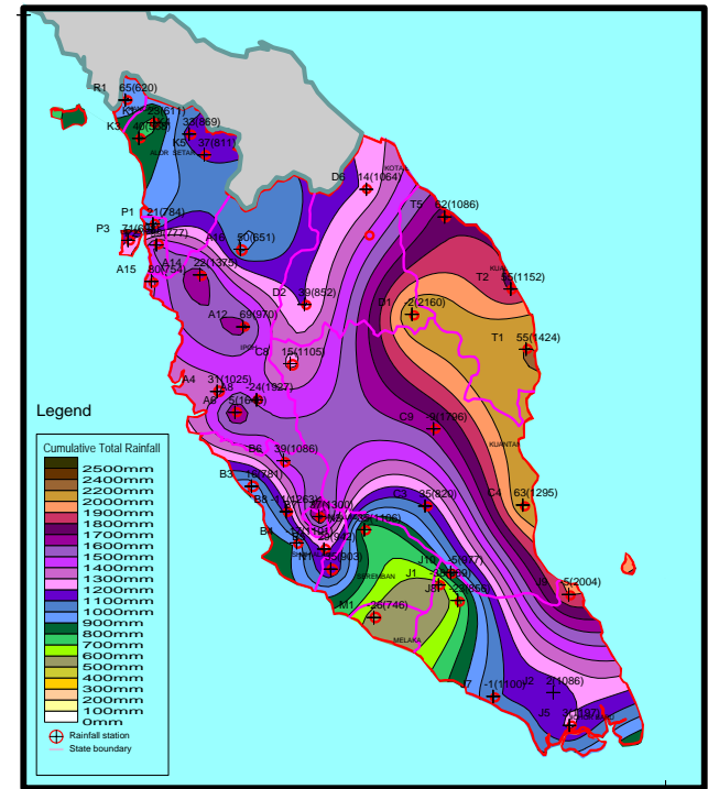
CUMULATIVE RAINFALL DISTRIBUTION IN PENINSULAR MALAYSIA YEAR 2009 PERIOD 6 month : 12_2008 & 1,2,3,4,5
