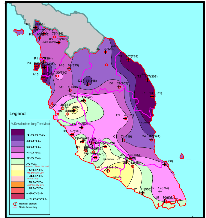
STATUS OF WATER RESOURCES In PENINSULAR MALAYSIA BASED On RAINFALL CUMULATIVE ANALYSIS YEAR 2009 PERIOD 3 month : 3,4,5
