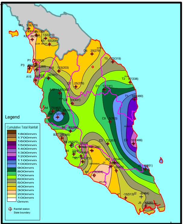
CUMULATIVE RAINFALL DISTRIBUTION IN PENINSULAR MALAYSIA YEAR 2009 PERIOD 3 month : 1,2,3
