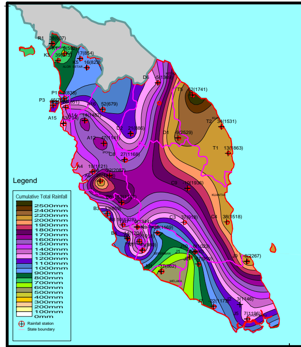
CUMULATIVE RAINFALL DISTRIBUTION IN PENINSULAR MALAYSIA YEAR 2009 PERIOD 6 month : 11,12_2008 & 1,2,3,4_2009
