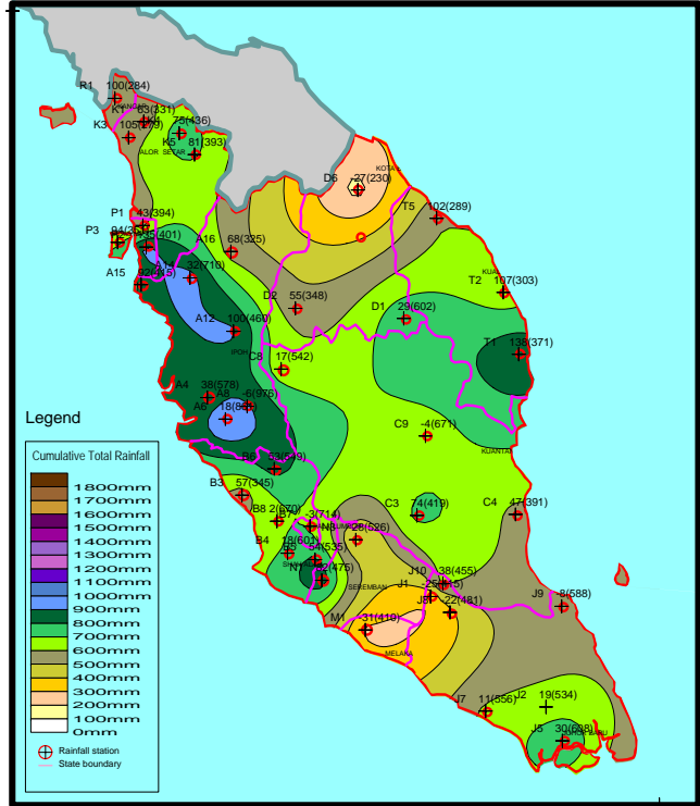
CUMULATIVE RAINFALL DISTRIBUTION IN PENINSULAR MALAYSIA YEAR 2009 PERIOD 3 month : 2,3,4
